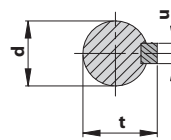
SHAFT DIMENSIONS
